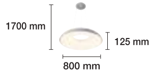
LÁMPARA COLGANTE DECORATIVA LED 80W REGULABLE
